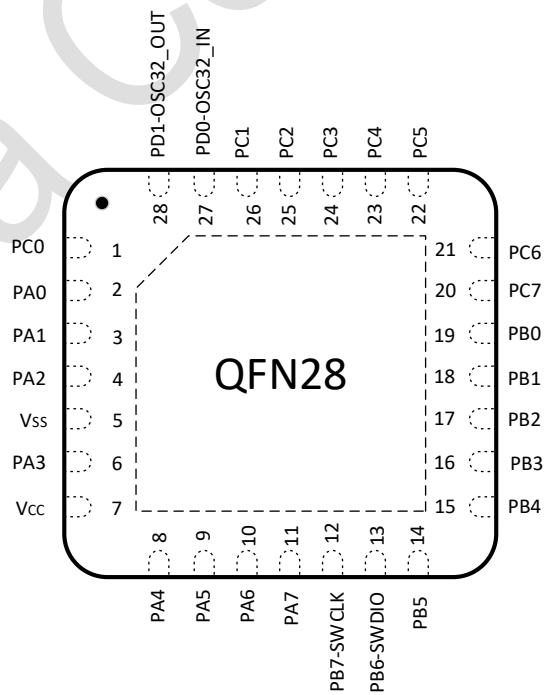
图 3-4 QFN28 Pinout1 PY32F005G1xU7
