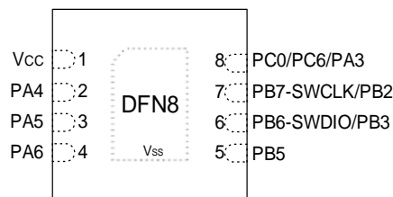
图 3-7 DFN8 (1.5*1.5) Pinout1 PY32F005L1xD7
